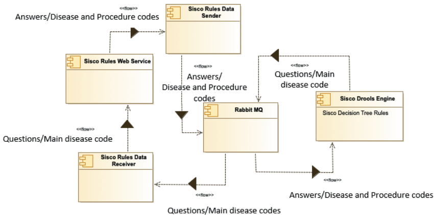
Figure 4: The Rules Engine Component Diagram.
