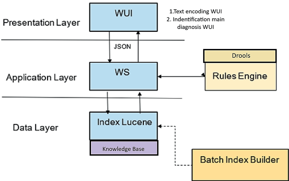
Figure 1: SISCO.web architecture.
